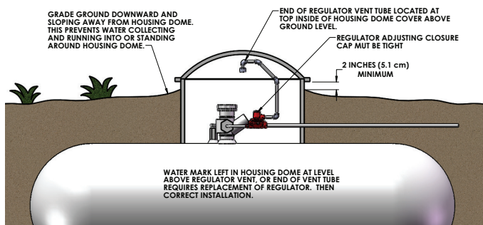
Figure 5: Underground Installation
